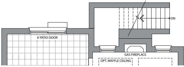
GROUND FLOOR W/OPT. BASEMENT SECONDARY SUITE ELEVATION A & B
