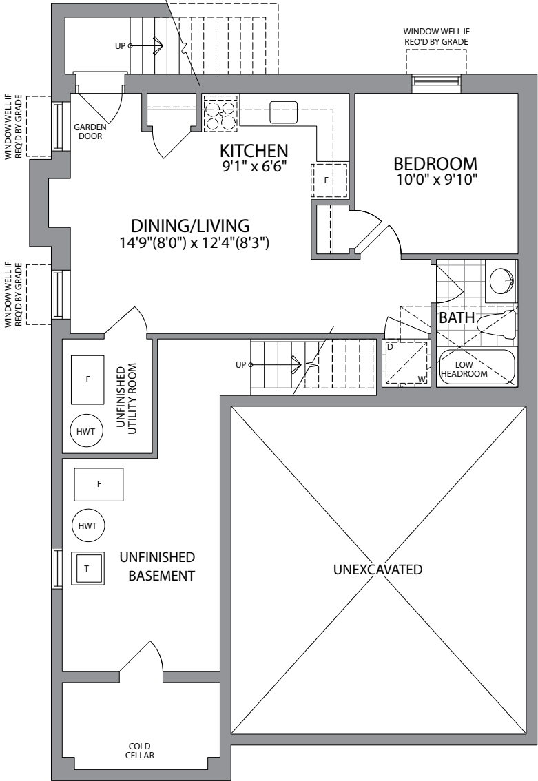
OPTIONAL BASEMENT W/SECONDARY SUITE ELEVATION A (B SIMILAR)
