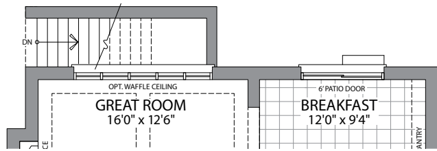
GROUND FLOOR, W/OPT. FINISHED BASEMENT ELEVATION A & B
