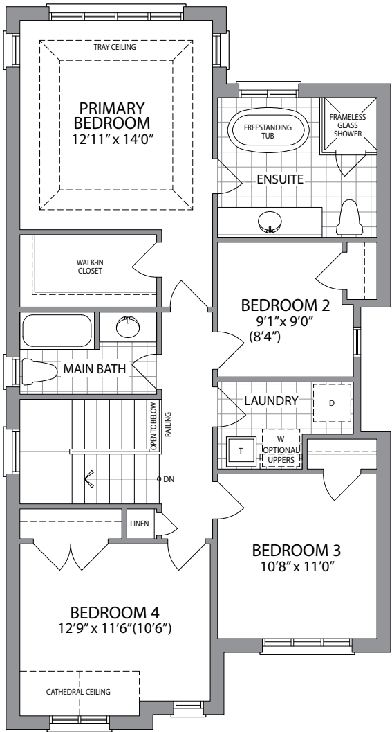
OPT. SECOND FLOOR ELEVATION A
