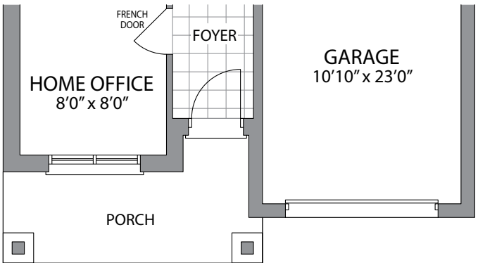
GROUND FLOOR ELEVATION B
