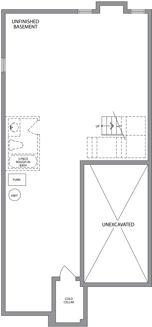
BASEMENT ELEVATION A & B
